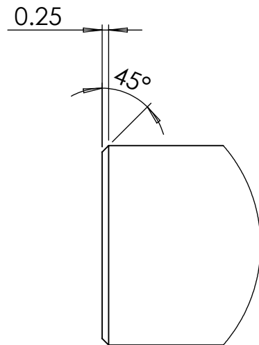
DETAIL A SCALE 5 : 1
